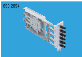
090.2694 FiberModul 7HP, plastic, breakout, 12xST multimode, PC, ceramic Артикул - R318909
