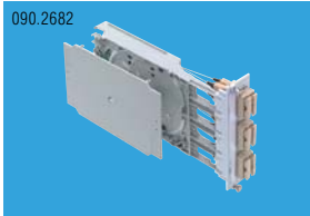
090.2682 FiberModul 7HP, plastic, splice, 6xSC-Duplex G.652.D, APC, ceramic, C/1 Артикул - R318965
