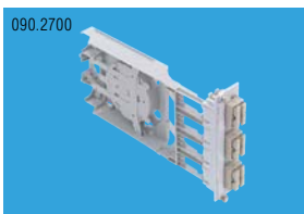
090.2700 FiberModul 7HP, plastic, breakout, 6xSC-Duplex singlemode, APC, ceramic Артикул - R318999
