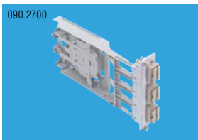
090.2700 FiberModul 7HP, plastic, breakout, 6xSC-Duplex multimode, PC, ceramic Артикул - R318914
