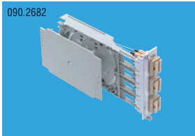
090.2682 FiberModul 7HP, plastic, splice, 6xSC-Duplex OM3, PC, ceramic, M/4 Артикул - R318900
