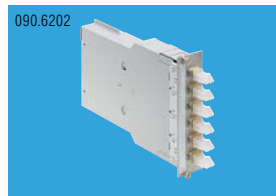
090.6202 MPO Modul 7HP, metal, MTP12-female - 6xLC-Duplex, OM4, PC/PC, ceramic, type A, серый Артикул - R514564
