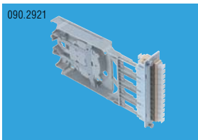
090.2921 FiberModul 7HP, plastic, breakout, 12xSC singlemode, APC, ceramic Артикул - R318989
